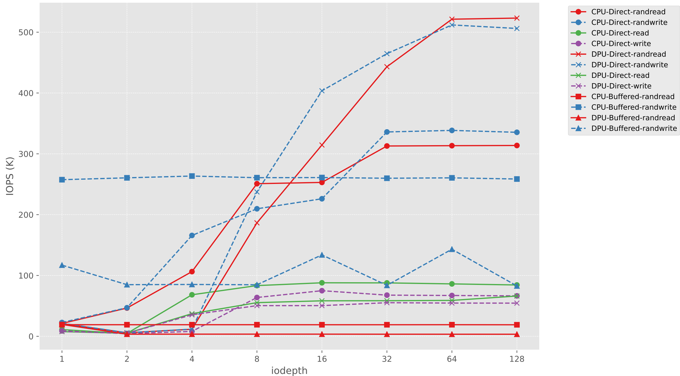
IOPS vs iodepth (CPU vs DPU, Direct vs Buffered)
